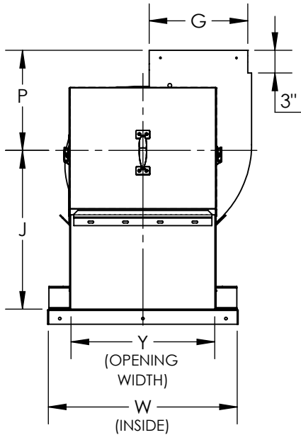
INLET VIEW
